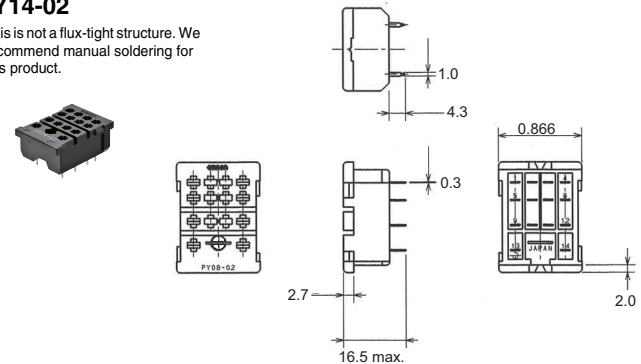
Terminal Arrangement/Internal Connection Diagram
