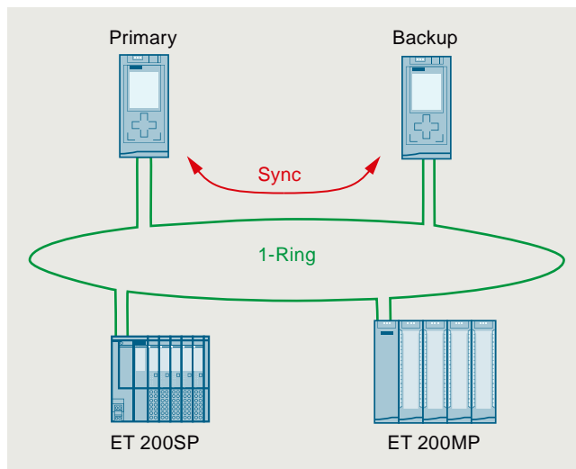
SIMATIC S7-1500R mode of operation
