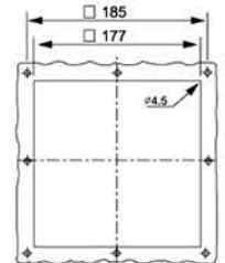
Drawing FKL 6623....
