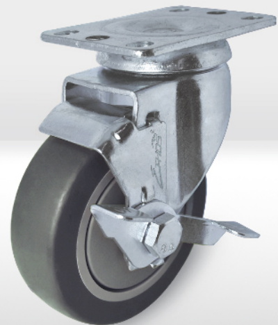
Side-Brake (Suffix 274) Top Plate 6 holes ready
