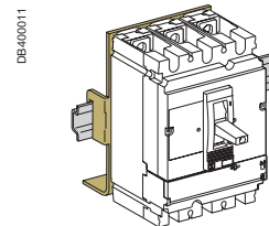
Mounting on DIN rail (with adaptor).
