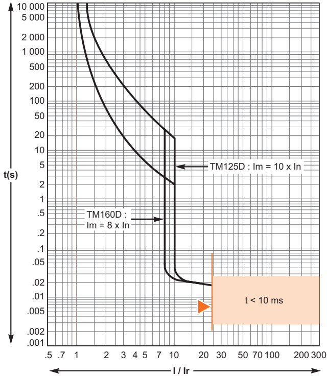
TM125D/160D
