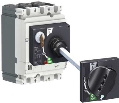
EasyPact EZS with an extended rotary handle installed at the back of a switchboard, with the keylock option and key.
