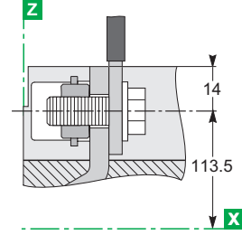
Bars/cables with lugs
