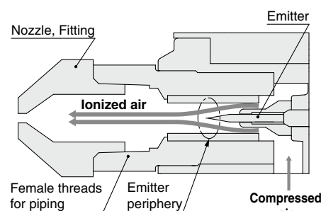
Sectional view of the female threads for piping
