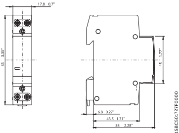
ESB16..N Dimensions mm, inches
