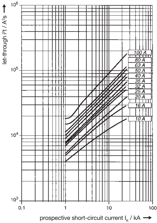
10 S 700 characteristic K_{selective} let-through energy
