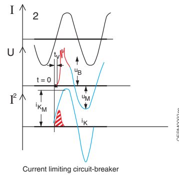
Short-circuit current
