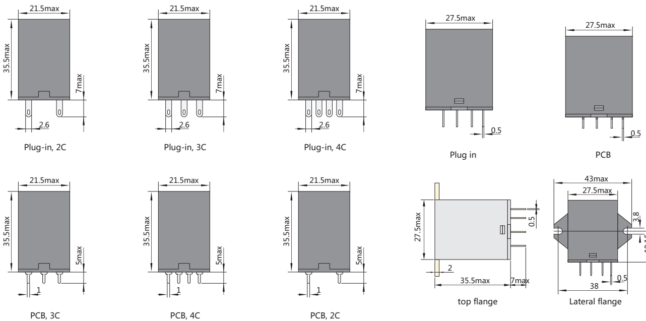
Left view
