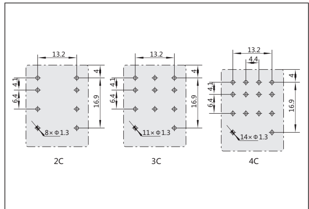
PCB mounting poles
