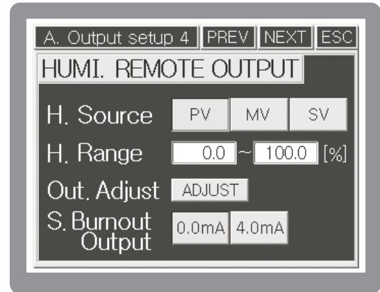
[Fig. 88] Humidity retransmission output setting screen.
