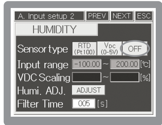
[Fig. 77] Humidity sensor setting screen
