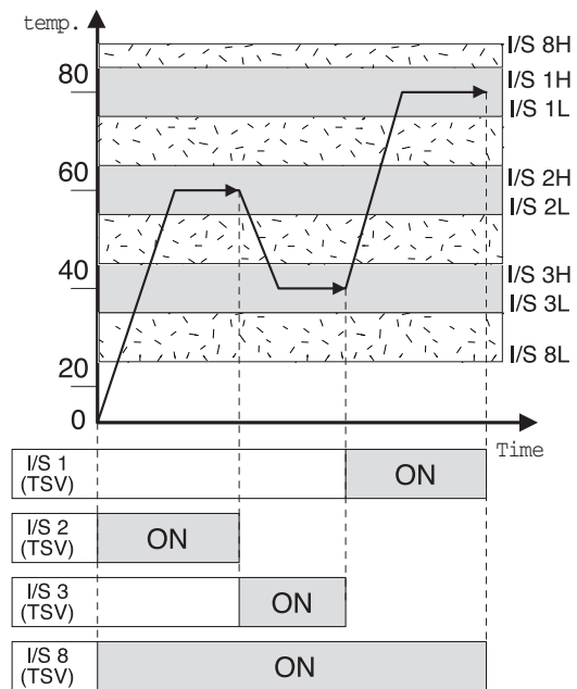
[Fig. 93] Example of Inner Signal setting (TSV)
