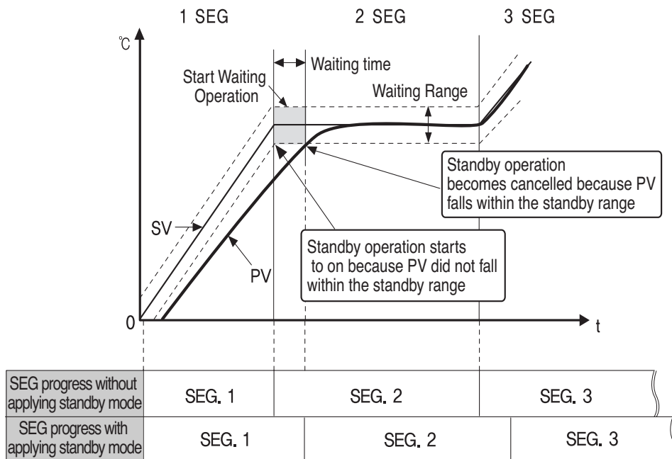
[Fig 57] Common waiting operation
