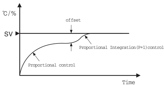
[FIG.107] Proportion (P) and Proportional Integration (P+I) control
