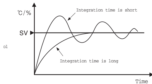
[FIG.108] Proportional Integration (P+I) control
