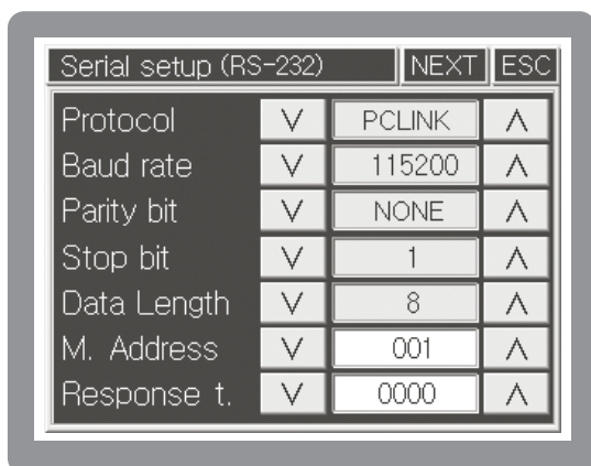
[FIG.120] Communication Parameter Setting (RS232)
