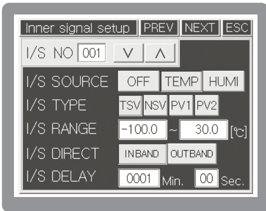
[FIG.131] Inner Signal Set
