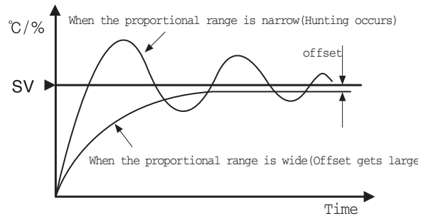
[FIG.106] Proportional control (P control)
