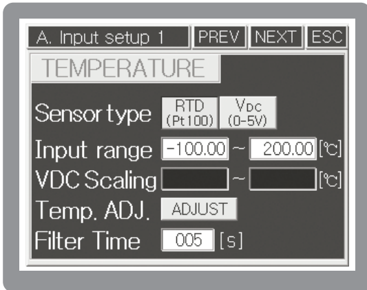
[Fig. 76] Temperature sensor setting screen
