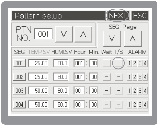
[Fig.49] Program Pattern Setting screen 1
