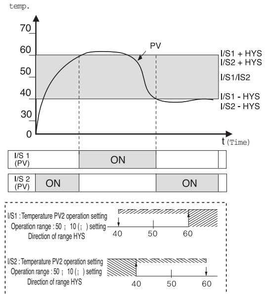
[Fig. 95] Example of Inner Signal setting (PV2)
