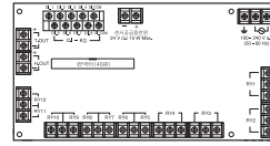
I/O Board 2
