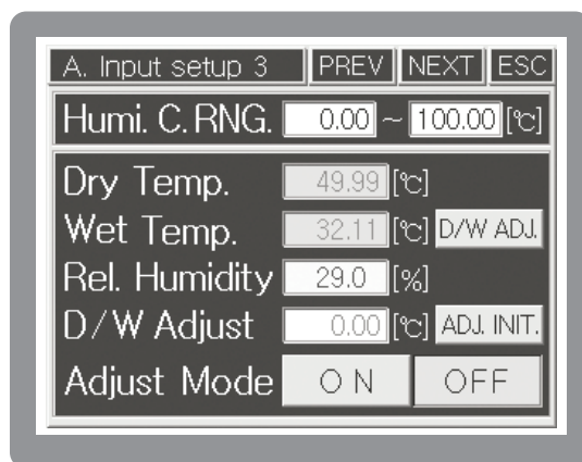
[FIG.81] Sensor Input Setting 3
