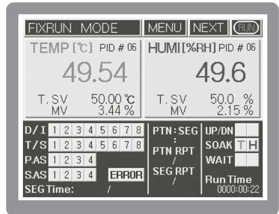
[Fig.15] Running screen 2 for Fix control
