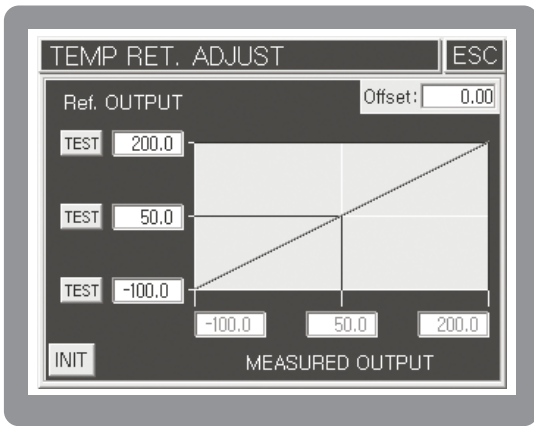
[Fig.89]Temperature retransmission output bias
