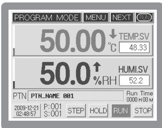
[FIG.142] Program control 1st operation screen
