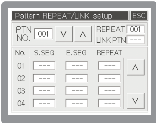
[FIG.140] Pattern repeat / Connection setting screen
