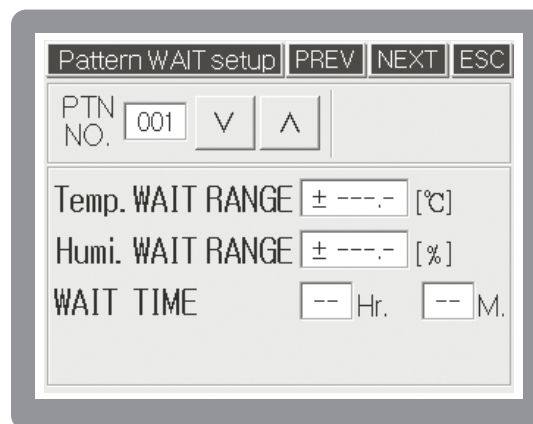
[Fig.56] Pattern WAIT setup screen
