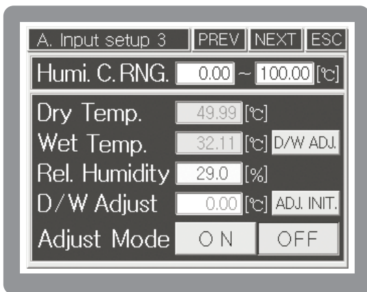
[FIG.126] Dry - Humidity sensor correction screen
