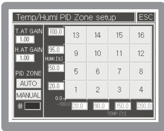
[Fig.102] Temp. & Humi P.I.D Zone Setting
