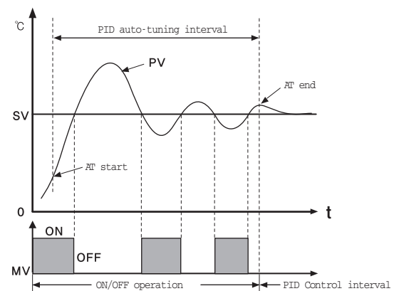
[Fig 22] PID Auto Tuning
