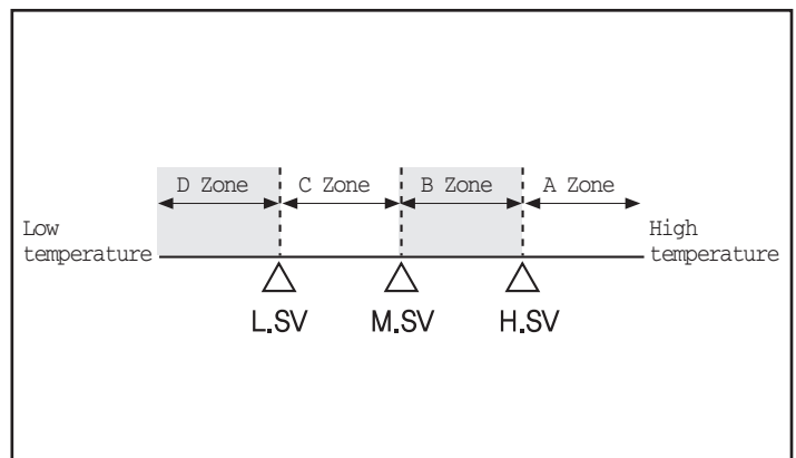
[Fig.97] Section of T ON/OFF zone
