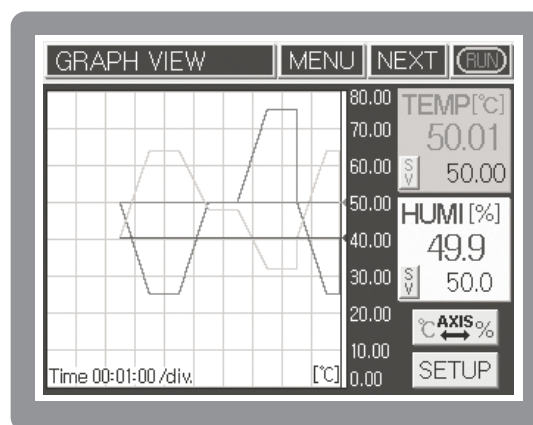
[Fig.24] Screen for program control graph display
