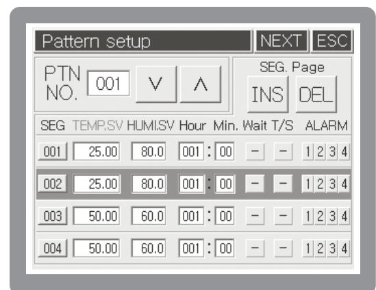
[Fig.47] Segment selection screen
