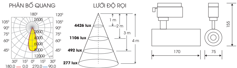
TRL08 10W (48V)
