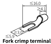
Fork crimp terminal
