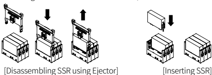
[Disassembling SSR using Ejector]
