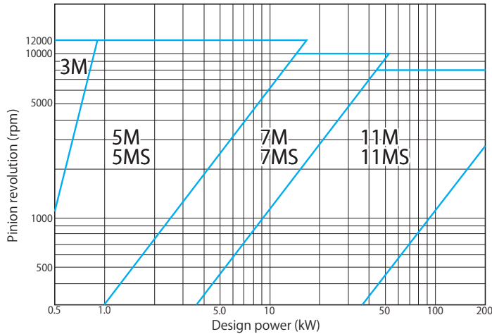
Fig. 1 Belt type selection diagram
